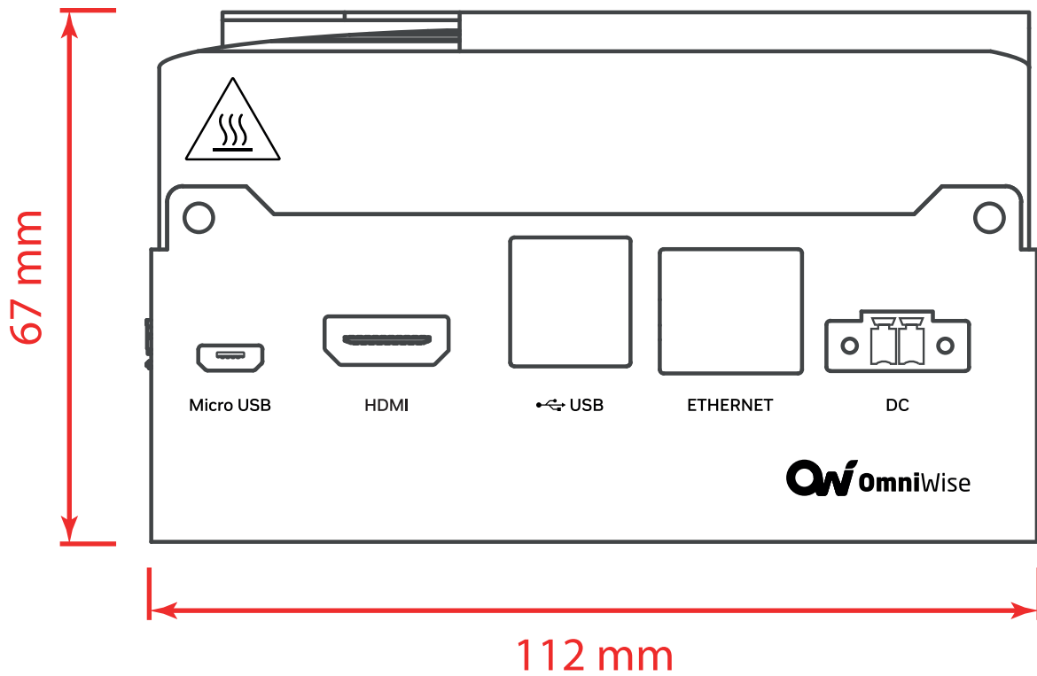
Front View Dimensions
